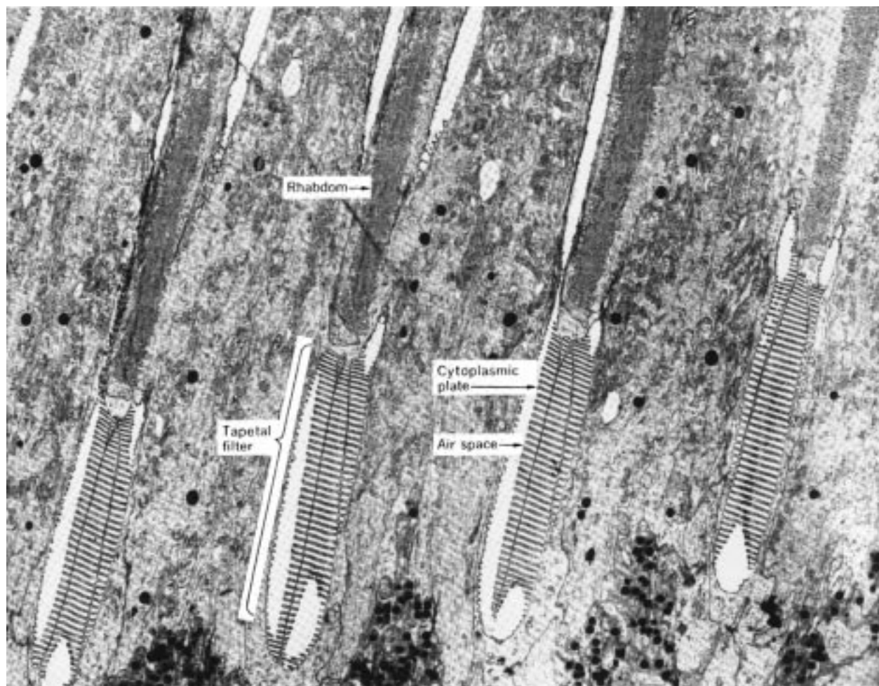
Figure 27. Electron micrograph of a section parallel to the ommatidial axis from a Buckeye butterfly eye. The periodicity of 0.23\ \mu\text{m} of the cytoplasmic plate leads to constructive interference, giving rise to the butterfly glow. (Reprinted with permission from ref 61a. Copyright 1970 The Institute of Electrical and Electronics Engineers, Inc.)
