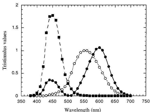
Figure 3. Color-matching functions of 1931 CIE standard 2° observer. The filled circles, open circles, and filled squares represent \bar{x} , \bar{y} , and \bar{z} , respectively. (Data from ref 18.)
